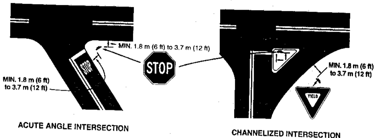
Figure 2A-2. Examples of Locations for Some Typical Signs at Intersections
