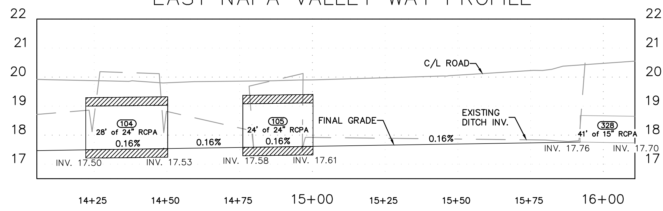
EAST NAPA VALLEY WAY PROFILE
