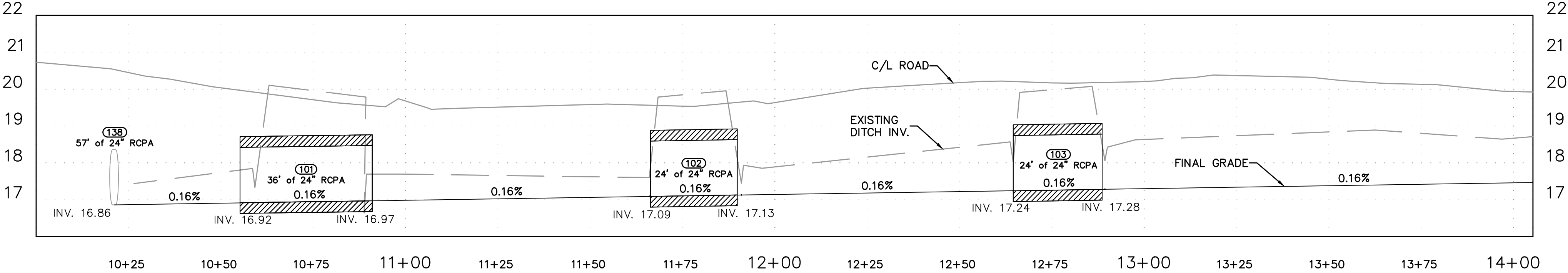
EAST NAPA VALLEY WAY PROFILE
