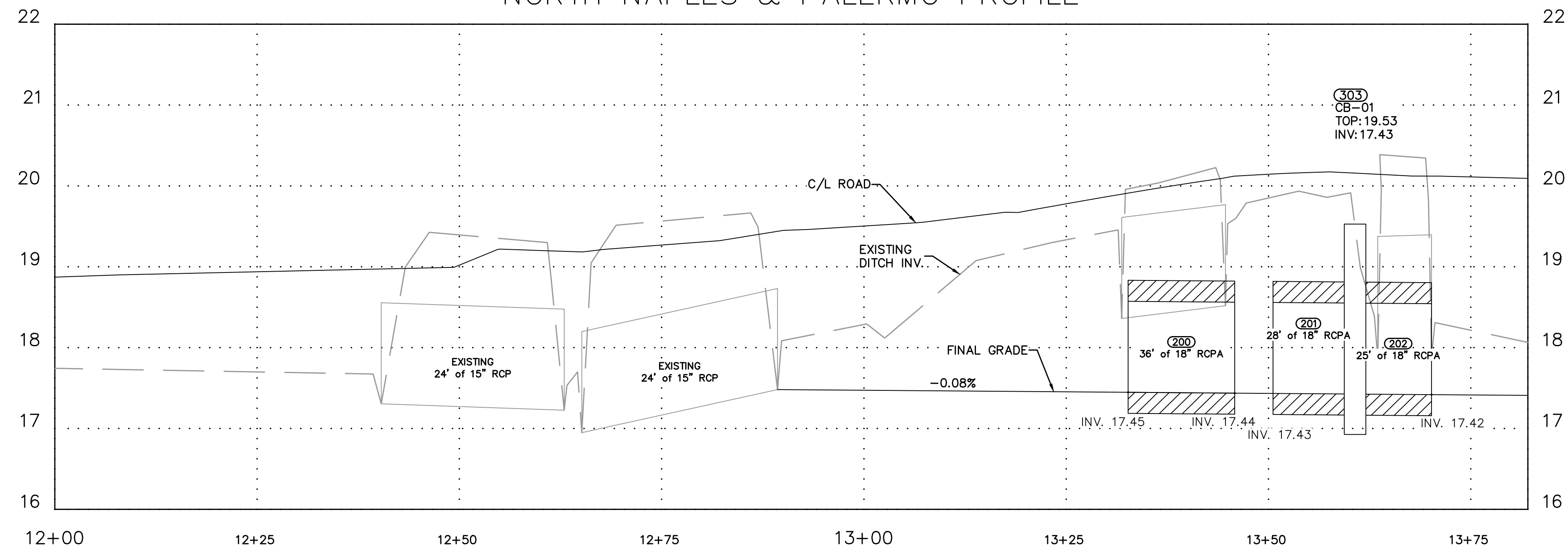
NORTH NAPLES & PALERMO PROFILE
